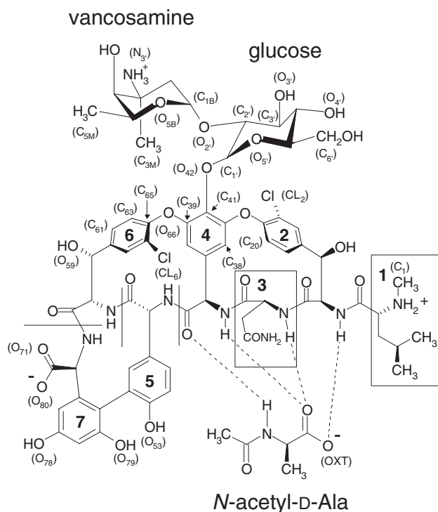
Figure 1. Chemical structure of vancomycin and the binding scheme between vancomycin and a cell-wall precursor analog, N -acetyl-D-Ala (AcDA). The amino acid residues of vancomycin are numbered. Atoms mentioned in the text are labeled. The hydrogen bonds between vancomycin and AcDA are shown by broken lines.
