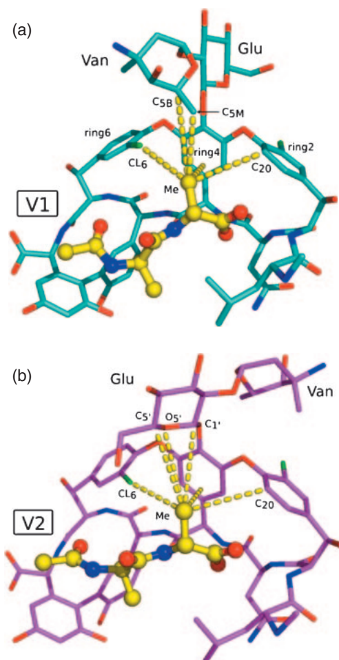
Figure 6. Multiple hydrophobic contacts between D-Ala methyl group of the ligand and the antibiotic molecule for V1 monomer (a) and V2 monomer (b) in the NAAA complex, 6 drawn with dotted lines.
