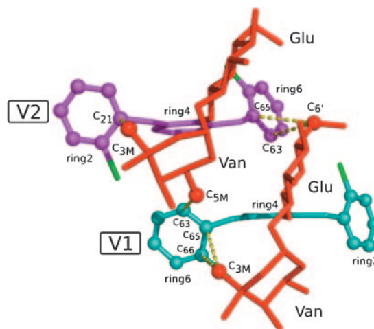
Figure 4. Hydrophobic contacts between sugars and aromatic rings at the back-to-back dimer-interface in the AcDA complex. The sugar–ring closest contacts of two intramonomer and two intermolecular pairs are drawn with dotted lines.
