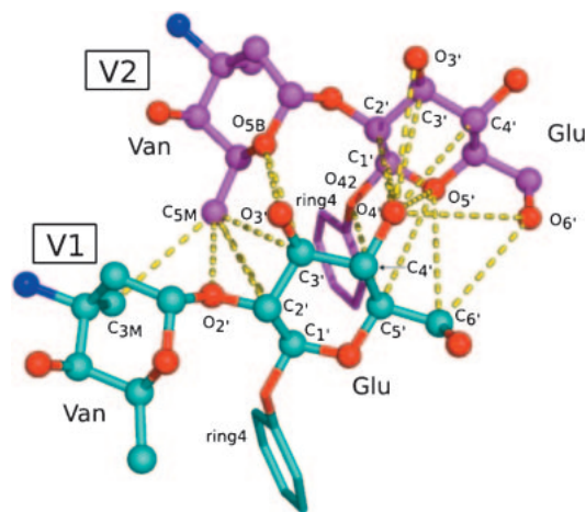
Figure 3. Close contacts ( <4.0 Å), drawn with dotted lines, between two parallel disaccharide chains at the back-to-back dimer-interface in the AcDA complex.
