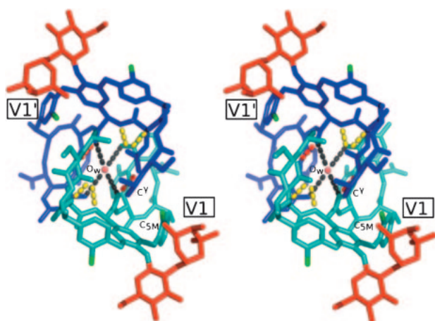
Figure 5. Stereoview showing the face-to-face arranged self-dimer V1–V1' in the AcDA complex. The dimeric structure is stabilized by direct or water-mediated hydrogen bonds between V1 and V1' monomers, shown in red or gray dotted lines, respectively, across a crystallographic dyad axis passing through the water molecule (pink sphere), the former being a pair of V1:3 N δ2 ...V1':4 O hydrogen bonds and the latter being two pairs of V1:4 O...O W ...V1':4 O and V1:7 O 79 ...O W ...V1':7 O 79 hydrogen bonds. Note that the Leu side-chain occupies the ligand-binding site of its dimer partner.
